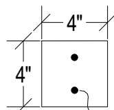
#3 REBAR (TYP.) 4" x 4" POST SECTION VIEW
