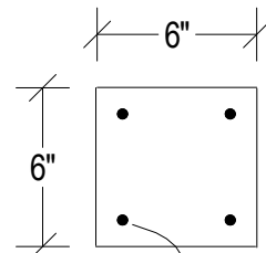
#3 REBAR (TYP.) 6" x 6" POST SECTION VIEW
